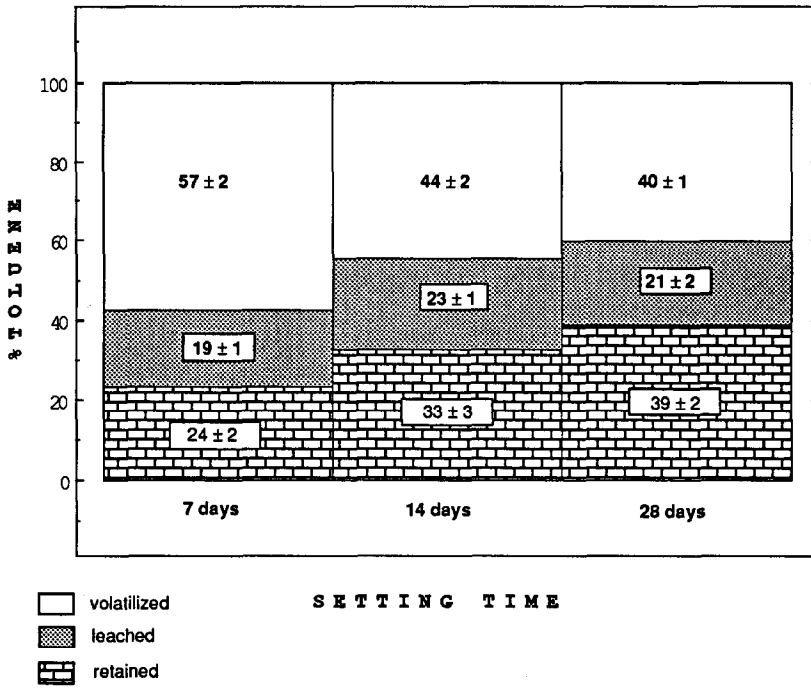
Fig. 4. Effect of setting time. Samples were prepared as 5% RHA, 4% OPC, and 7% water.
